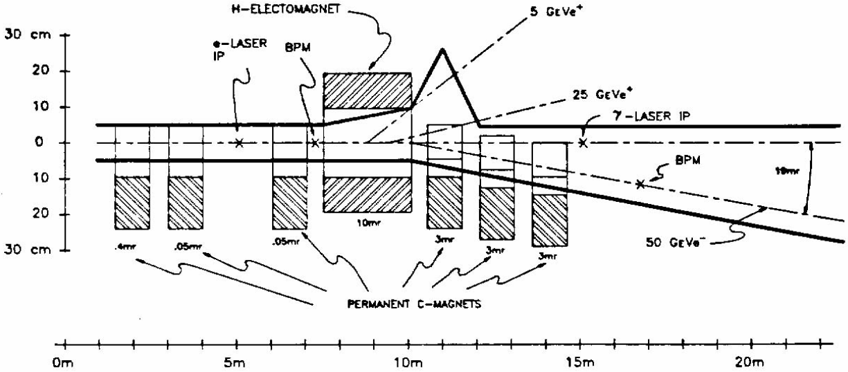
ELEVATION: DUMP MAGNETS AND VACUUM VESSEL FOR QED EXPERIMENT IN THE FFTB
