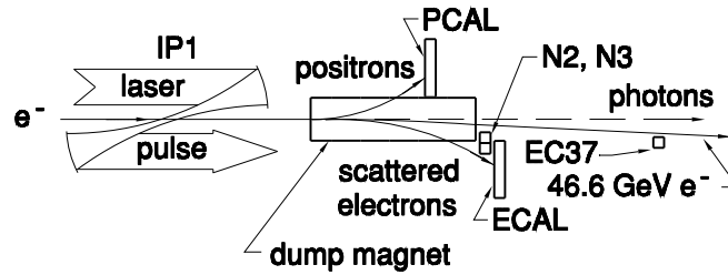
Figure 7. Layout of SLAC E-144 in which a terawatt laser collides at 17^\circ with a 46.6 GeV electron beam to produce backscattered photons, electrons and positrons via nonlinear QED processes.
