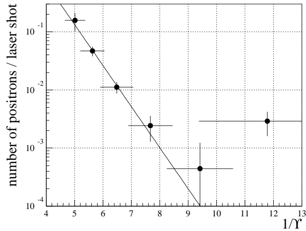
Figure 13. The observed rate of positron production vs. 1/\Upsilon .
