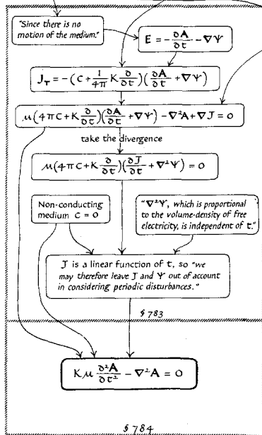
FIG. 3. Maxwell's derivation of the wave equations in the Treatise on Electricity and Magnetism, 2nd Ed.
