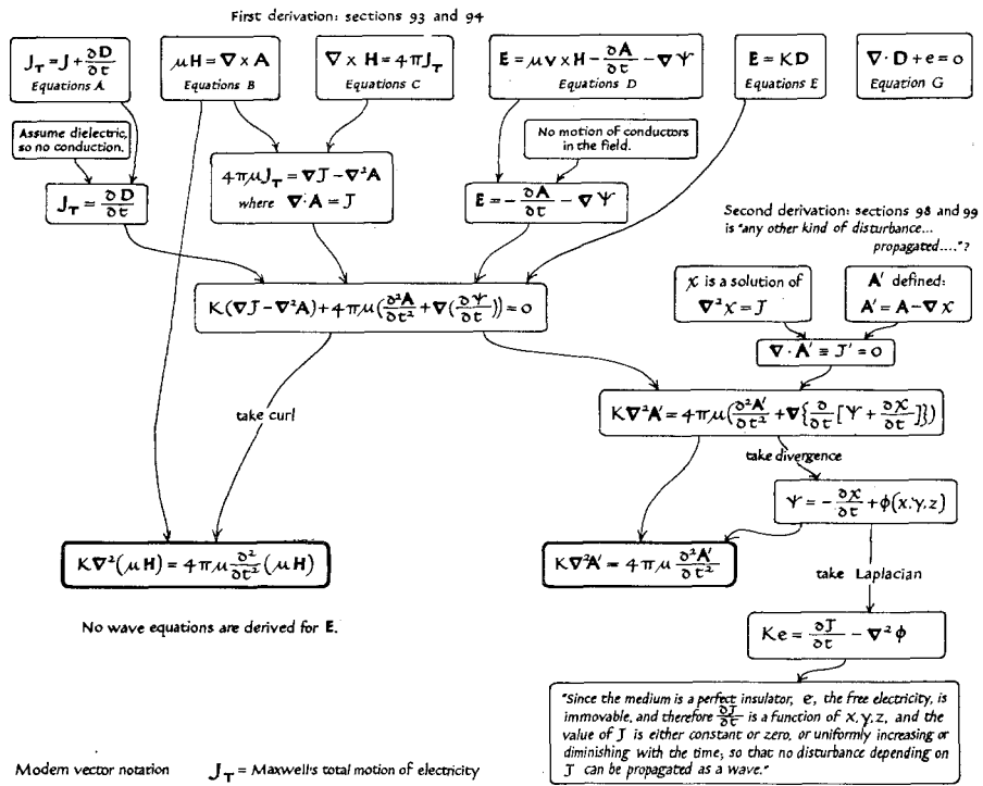
FIG. 1. Maxwell's derivation of the wave equations in "A Dynamical Theory of the Electromagnetic Field."
