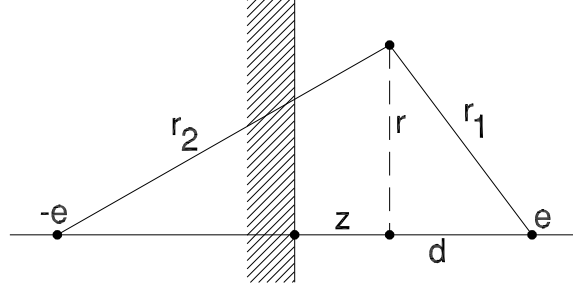
Figure 1: The charge e and its image charge -e at positions (r, \theta, z) = (0, 0, \pm d) with respect to a conducting plane at z = 0 . Vectors \mathbf{r}_1 and \mathbf{r}_2 are directed from the charges to the observation point (r, 0, z) .
