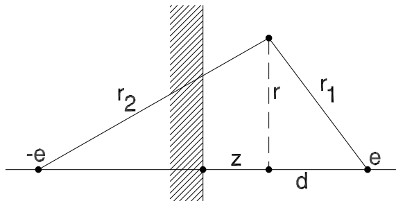
Figure 1: Electric charge e and its image charge -e at positions (r, \theta, z) = (0, 0, \pm d) with respect to a conducting plane at z = 0 . Vectors \mathbf{r}_1 and \mathbf{r}_2 are directed from the charges to the observation point (r, 0, z) .
