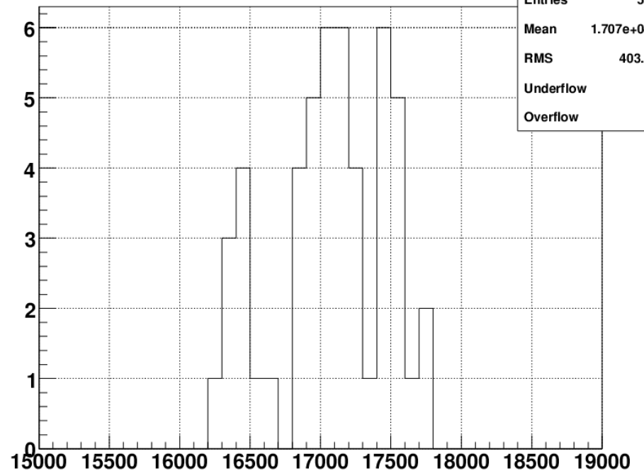
\mu^- distribution 9 GeV – ST2 – 40 < E_{kin} < 180 MeV/c
