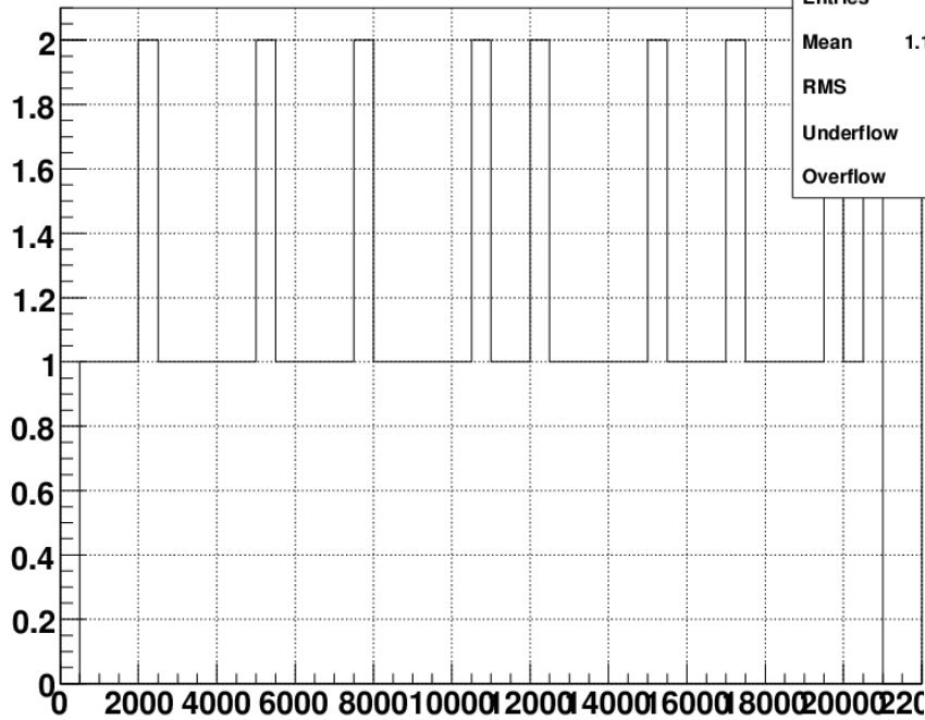
v_\mu distribution 9 GeV – ST2
