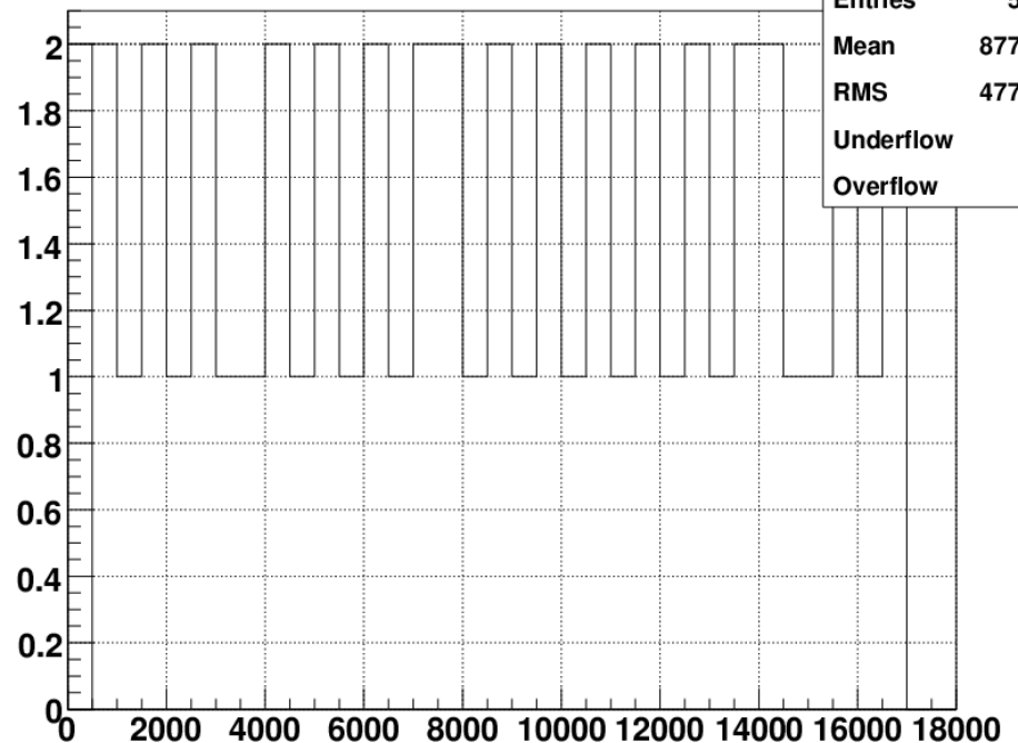
v_\mu bar distribution 9 GeV – ST2
