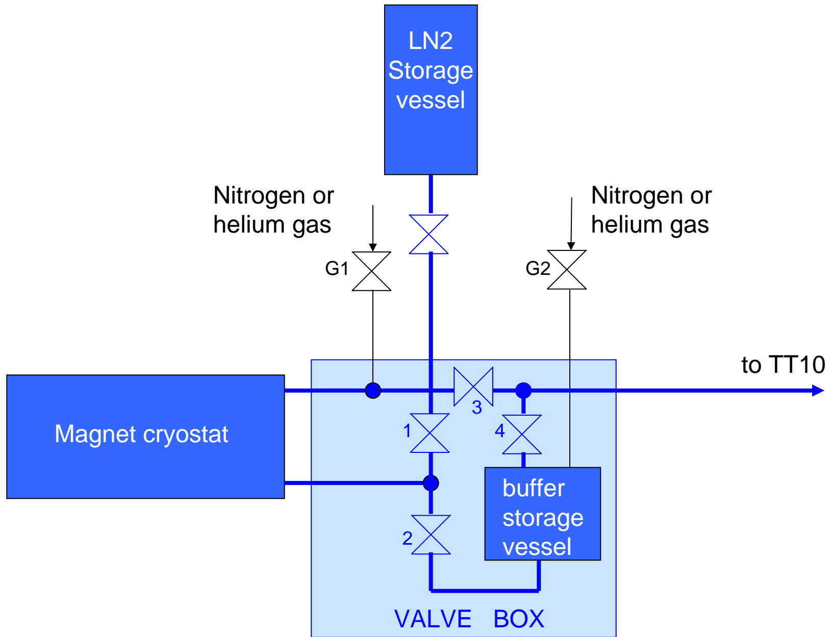
Schematic diagram of the cryogenic system
