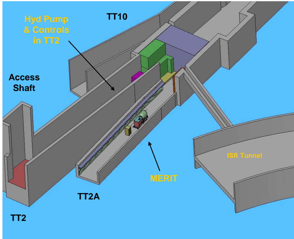
Figure 32. MERIT layout in the CERN tunnels.
