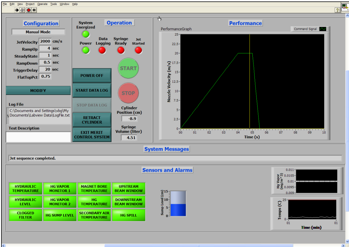
Figure 33. Labview control system operator interface
