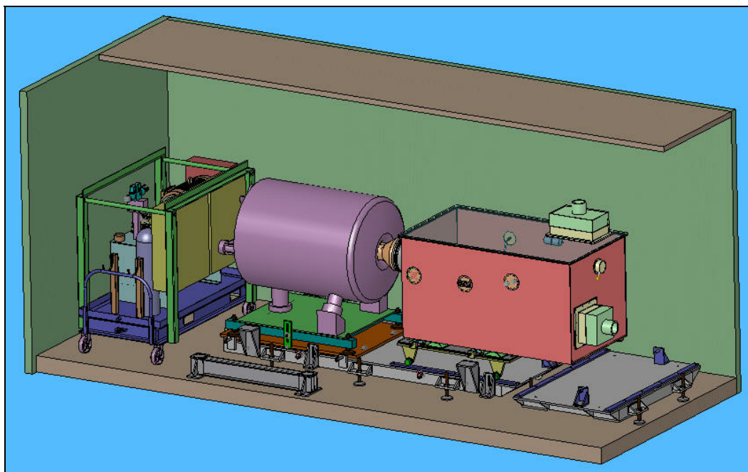
Figure 38. Target equipment and solenoid inside a short sealand container.
