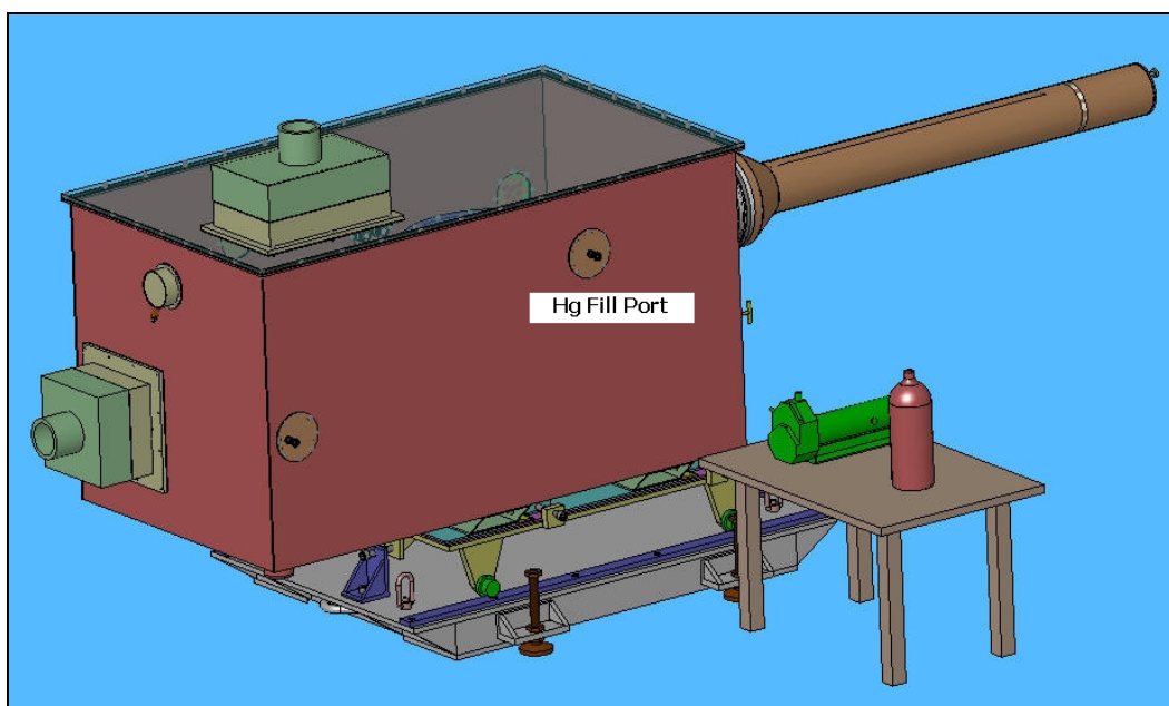
Figure 34. Mercury fill port.
