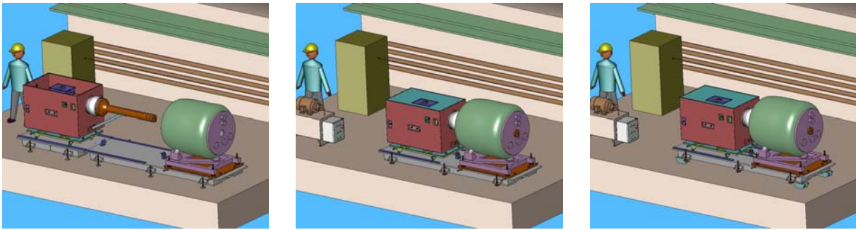
Figure 37. Target equipment inserted into solenoid.
