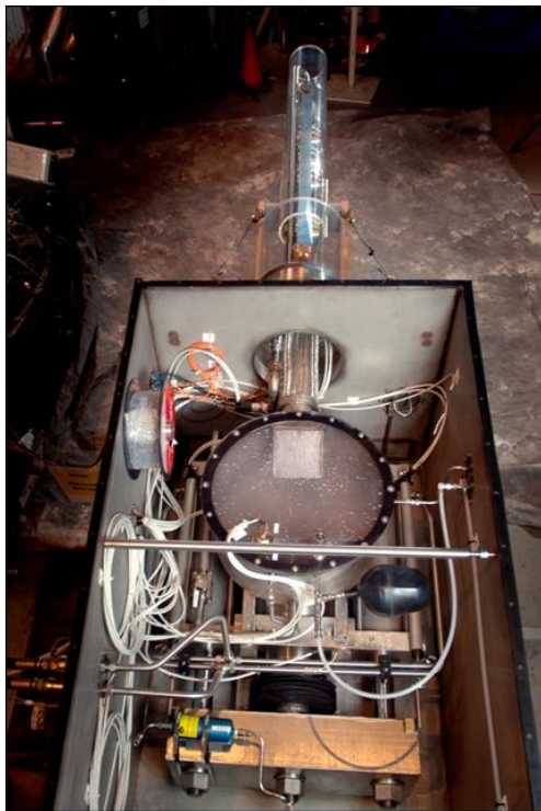
Figure 3. Hg delivery system.
