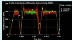
LS-DYNA result for a tungsten wire
