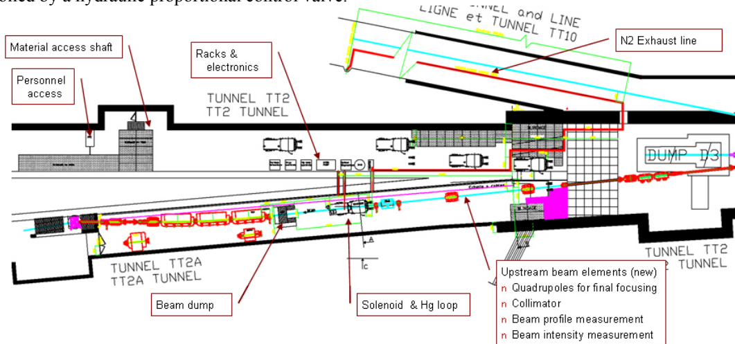
Figure 2. MERIT experimental layout in CERN TT2/TT2A tunnels.
