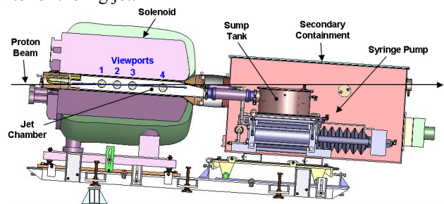
Figure 1: Vertical cross-section of MERIT equipment.
