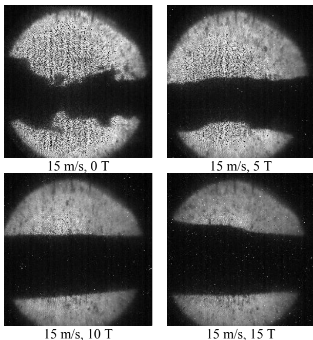
Figure 3. Influence of magnetic field on jet profile.
