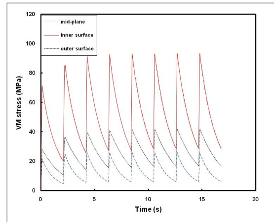
Figure 5: Transient stress at beam centre as a result of temperature cycling.
