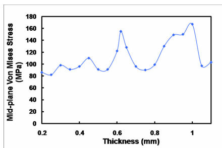
Figure 7: Window max stress with varying thickness.
