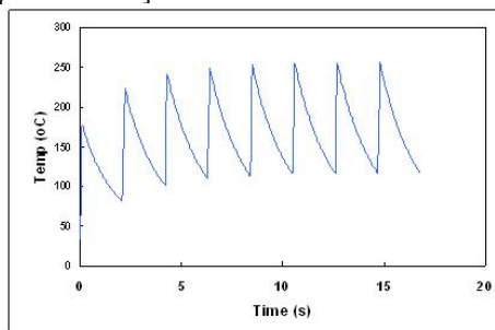
Figure 4: Temperature cycling between pulses at beam centre.
