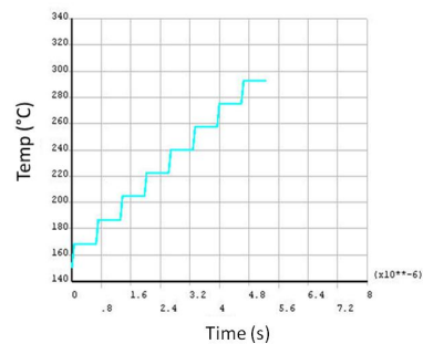
Figure 3: Temperature of window at beam centre over pulse duration
