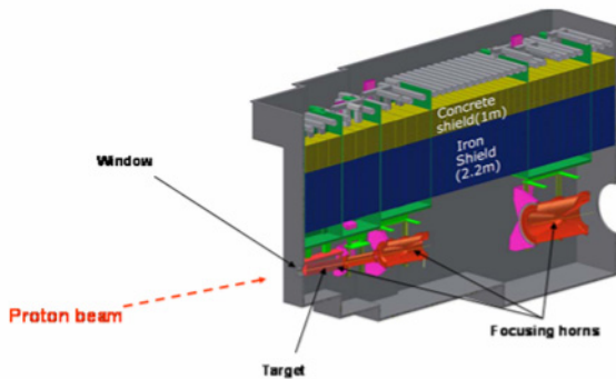
Figure 1: Target station layout.
