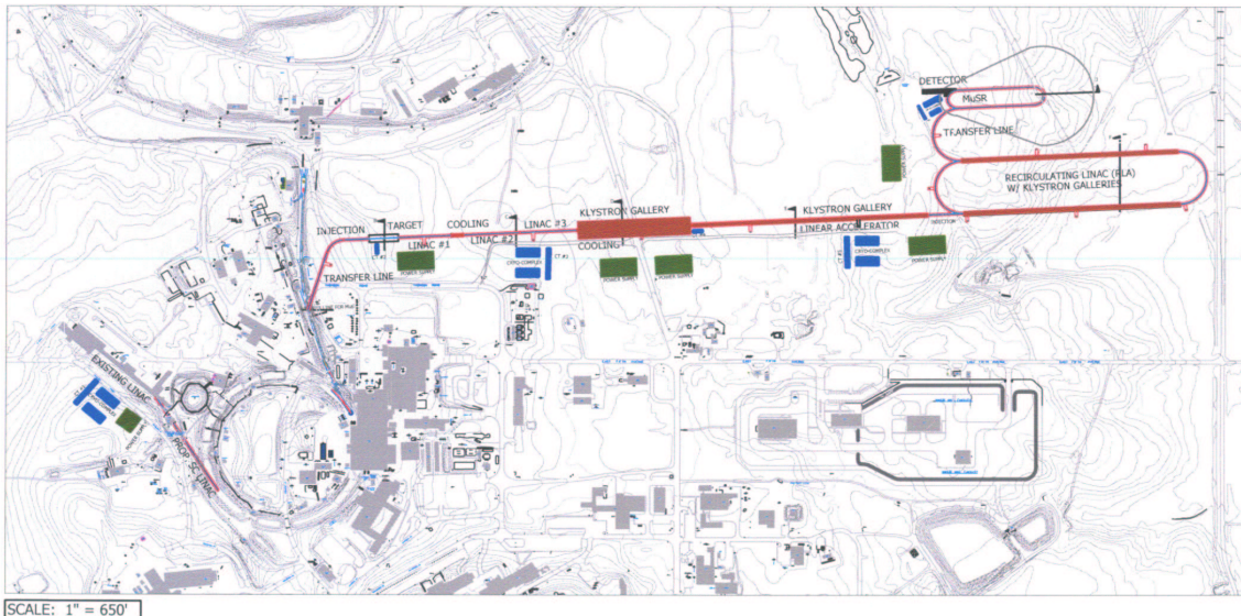
NEUTRINO FACTORY, SITE PLAN
