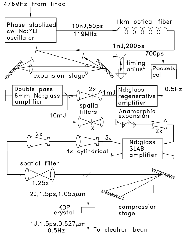
FIG. 7. Sketch of the terawatt Nd:glass laser system.
