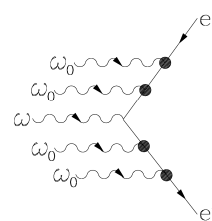
FIG. 3. Diagram representing multiphoton pair creation.
